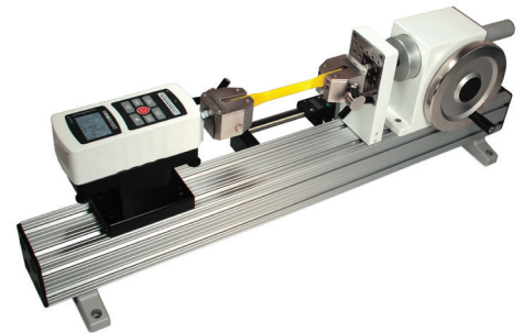
The TSFH is shown configured for a tensile test, with Series 5 digital force gauge, film and paper grips, and digital travel display
